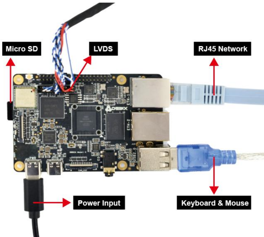
Figure 24 Hardware connection
