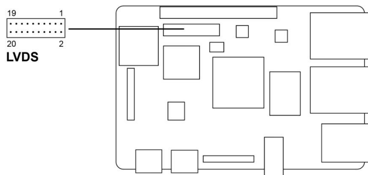
Figure 8 LVDS Interface
